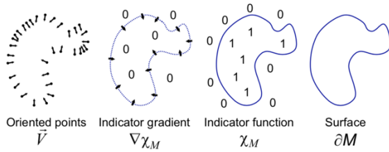
Figure 7: Stages of Poisson Reconstruction in 2D
