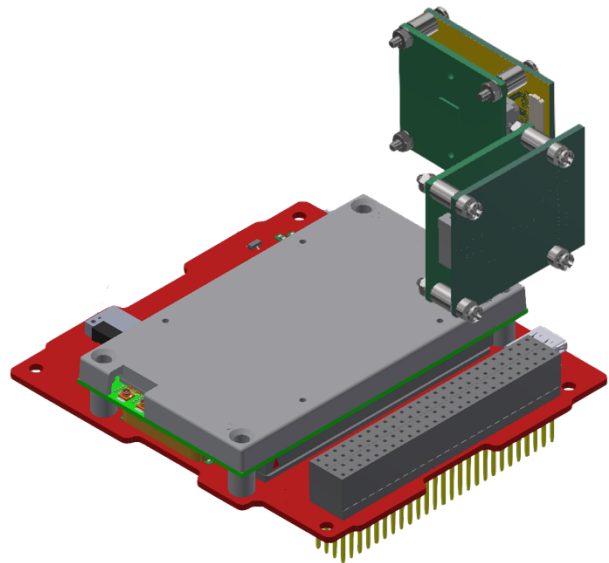
Figure 2: Payload Electronics
